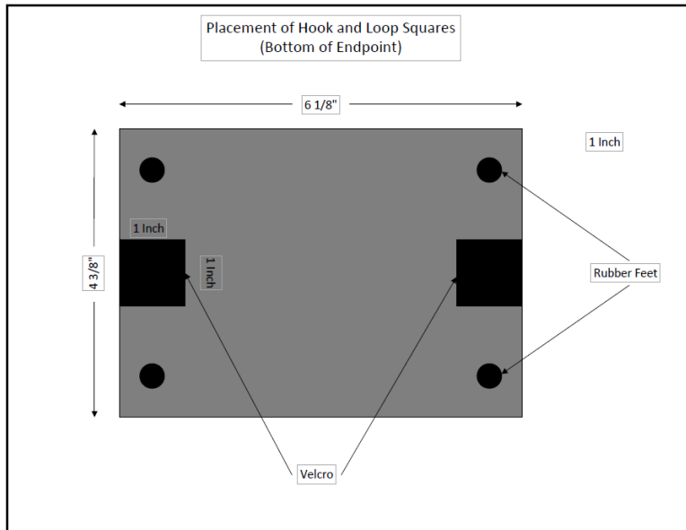
Velcro Mounting Diagram
